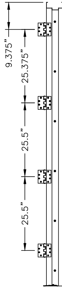
HINGE LOCATIONS 2" HEAD
