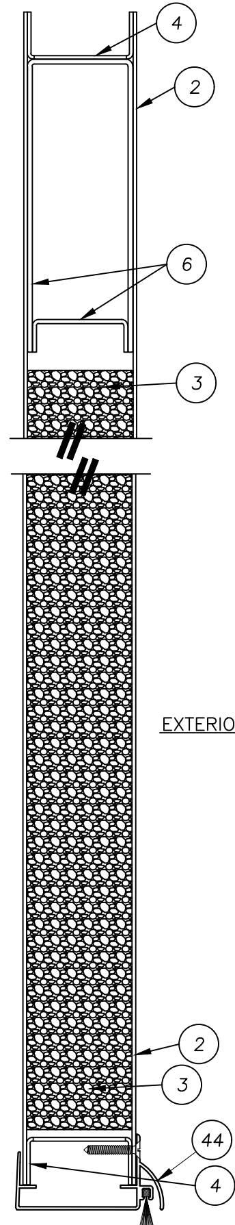
1 2 VERTICAL CROSS SECTION
